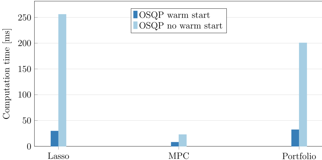
Figure 4: OSQP warm start and factorization caching benchmarks.
