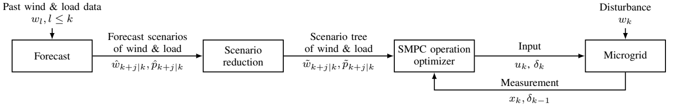
Fig. 1. Forecast with scenario reduction, scenario-based stochastic MPC (SMPC) and MG.
