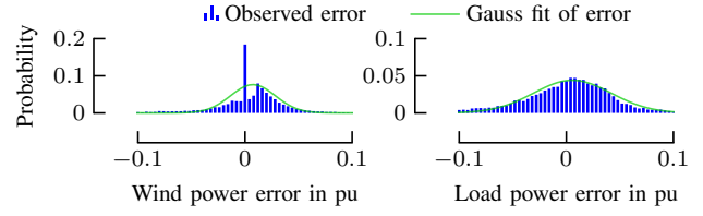
Fig. 3. Error distribution of all SARIMA( \chi_p, d, \chi_q, s, \chi_P, \chi_Q ) load and ARIMA( \chi_p, 0, \chi_q ) wind power forecasts. The peak at 0 pu in wind power is due to the saturation for wind speed lower 2.5 m/s and higher 12 m/s.
