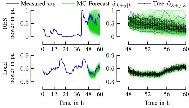
Fig. 2. Wind forecast with ARIMA( \chi_p, 0, \chi_q ) and load prediction with SARIMA( \chi_p, d, \chi_q, s, \chi_P, \chi_Q ) model over a horizon of 12 h. The scenario fan was generated using MC simulations with 500 seeds. The scenario tree was determined using a branching factor b = (8, 2, 2, 1, \dots, 1) .
