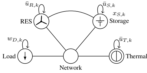
Fig. 4. Microgrid considered for case study.
