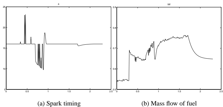
Figure 10. Nonlinear model + RHC controller + noise on torque measurements
