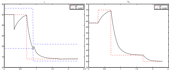
(a) Air-to-Fuel Ratio (dashed line: desired value, solid line: response of the nonlinear model, dash-dotted lines: constraints) (b) Intake Manifold Pressure (dashed line: desired value, solid line: response of the nonlinear model)
