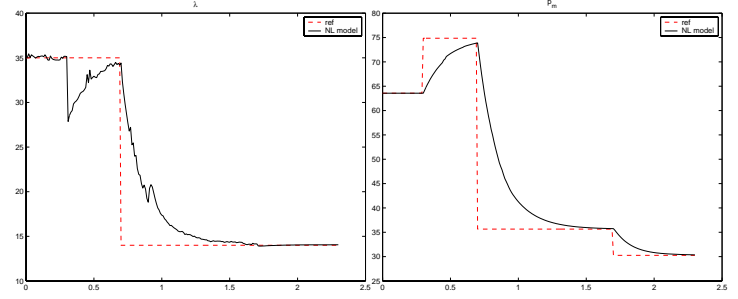
(a) Air-to-Fuel Ratio (dashed line: desired value, solid line: response of the nonlinear model) (b) Intake Manifold Pressure (dashed line: desired value, solid line: response of the nonlinear model)
