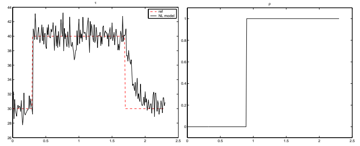
(a) Engine brake torque (dashed line: desired value, solid line: response of the nonlinear model) (b) Regime of combustion
