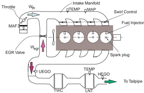
Figure 1. Direct Injection Stratified Charge (DISC) Engine.
