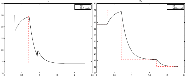
(a) Air-to-Fuel Ratio (dashed line: desired value, solid line: response of the MLD model)
