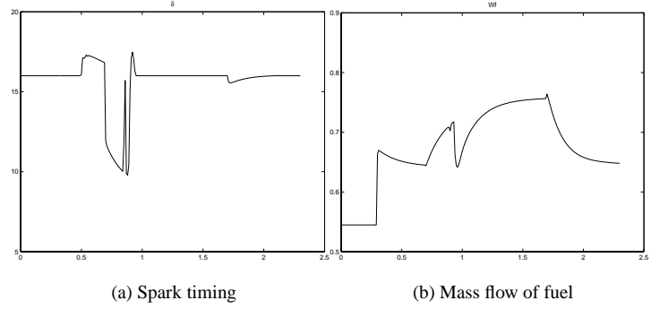
Figure 4. Nominal performance (MLD model + RHC controller)
