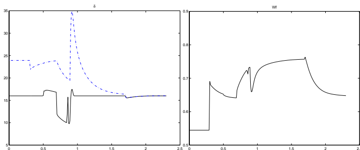
(a) Spark timing (solid line: actual value, dashed line: upper constraint (lower constraint is zero)) (b) Mass flow of fuel
