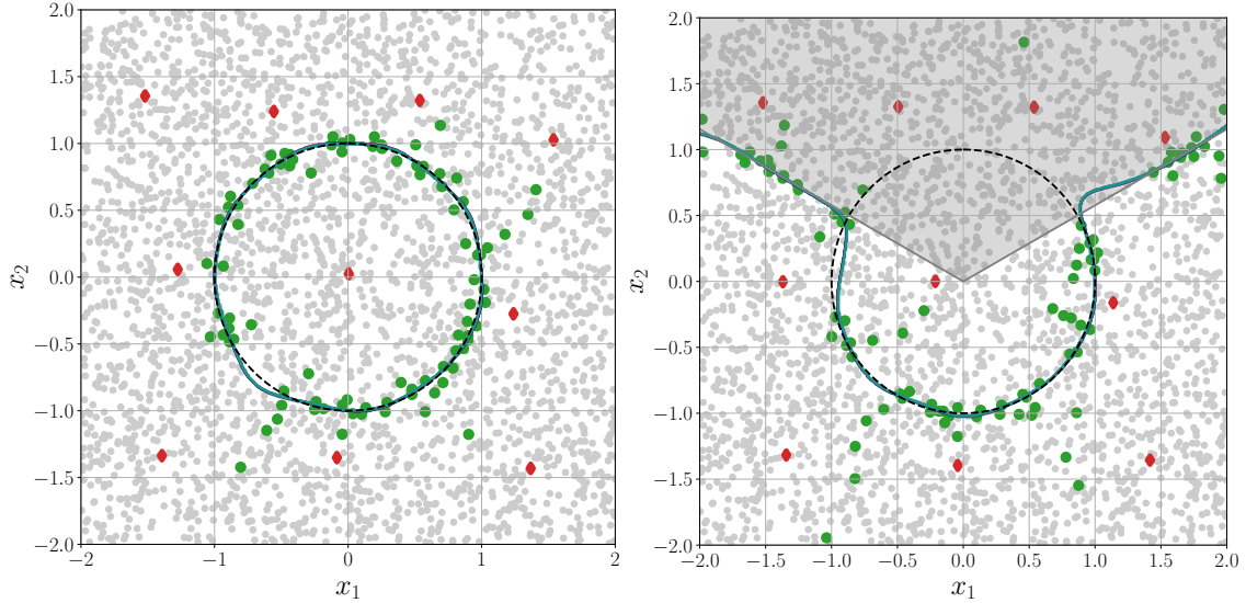
Figure 6: Classification problem (18), with and without the unknown constraint (19): decision boundary of learned classifier (blue curve), pool \mathcal{X}_P (gray circles), queried samples (green dots), initial samples (red diamonds), indicator function (dashed black line)
