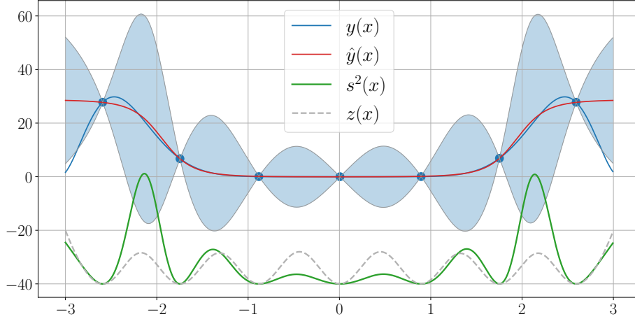
Figure 1: Example 3.1: function y (blue line), samples (x_k, y_k) (blue dots), NN predictor \hat{y} (red line), band \hat{y}(x) \pm 3\sqrt{s_i^2(x)} (light blue area), scaled and shifted IDW functions s^2 (green line) and z (dashed gray line)
