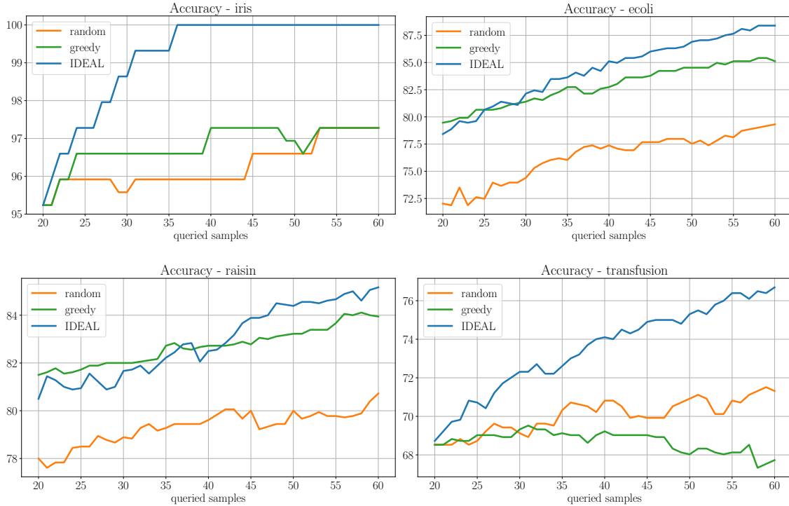
Figure 8: Classification problems, median accuracy results: iris (upper left), ecoli (upper right), raisin (lower left), transfusion (lower right)
