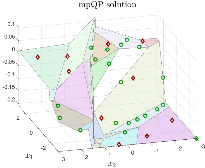
Figure 4: mpQP problem ( m = 2 ): exact mpQP solution, queried samples (green circle) and initial samples (red diamonds)
