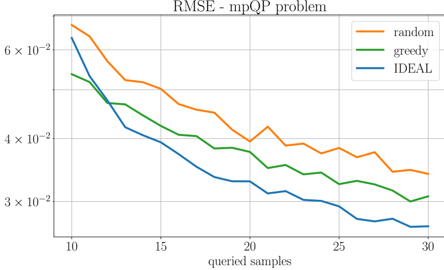
Figure 3: mpQP problem ( m = 2 ): median RMSE as a function of the number of queries
