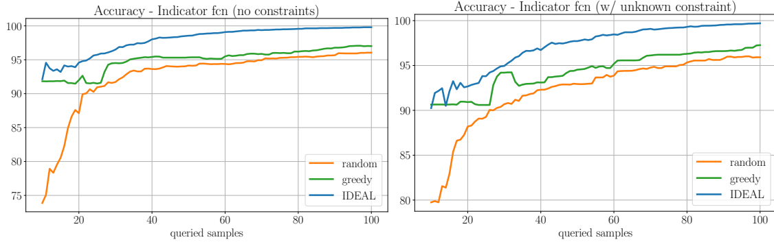
Figure 5: Classification problem (18), median accuracy without (left plot) and with unknown constraint (19) (right plot)
