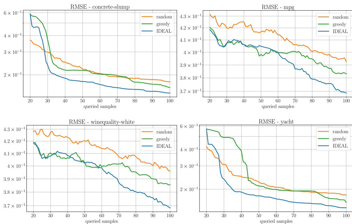
Figure 7: Regression problems, median RMSE results: concrete-slump (upper left), mpg (upper right), winequality-white (lower left), yacht (lower right)
