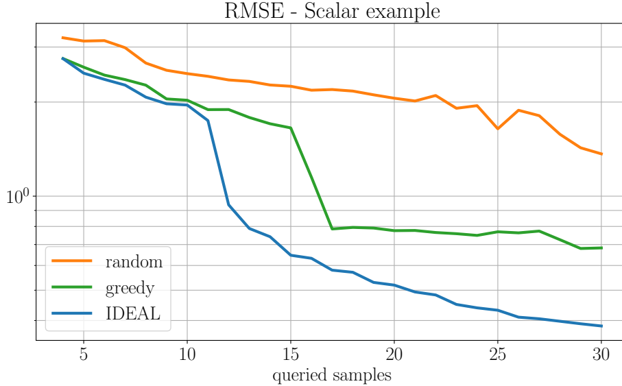
Figure 2: AL of function (11): median RMSE as a function of the number of queries
